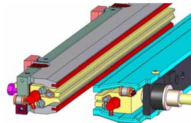
EZseal Sealing System for Polyethylene eliminates the need for tape.
