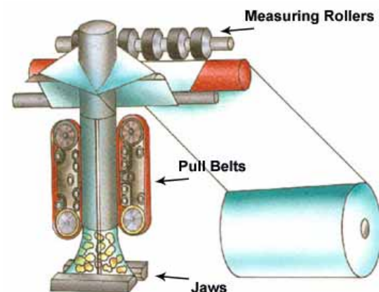
HayssenSandiacre's patented Measure, Form, Pull system is the fastest, production-proven way to package food.
